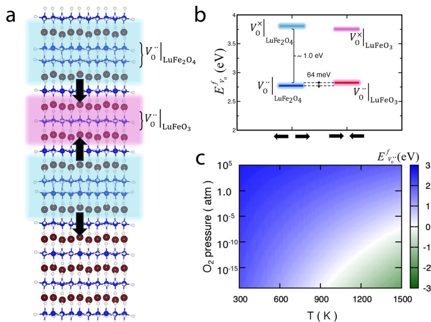
Fig. 3 | Defect formation energy for oxygen vacancies in LuFe 2 O 4 and LuFeO 3 . a Crystal structure of the (LuFeO 3 ) 3 /(LuFe 2 O 4 ) 1 superlattice, illustrating the local tail-to-tail and head-to-head polarization configurations (see also Fig. 1a). b The formation energy of oxygen vacancy at the oxygen-rich limit and for E_F = 0 (which corresponds to the valence band maximum). V_{O|\text{LuFe}_2\text{O}_4}^{\times} ( V_{O|\text{LuFeO}_3}^{\times} ) and V_{O|\text{LuFe}_2\text{O}_4}^{\cdot\cdot} ( V_{O|\text{LuFeO}_3}^{\cdot\cdot} ) correspond to oxygen vacancies in 2+ and neutral charge states in the
