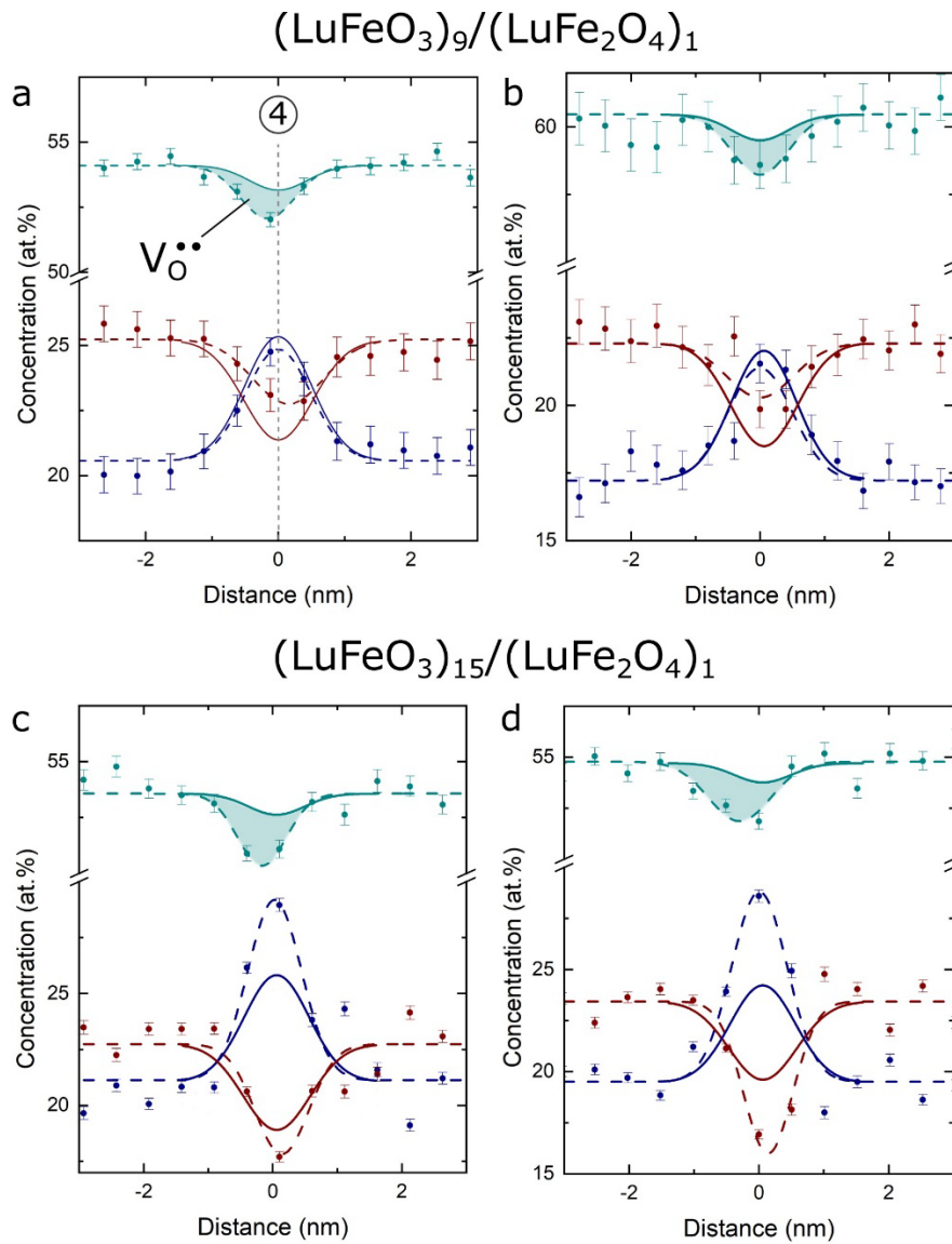
Figure S2: APT analysis of additional (\text{LuFeO}_3)_m/(\text{LuFe}_2\text{O}_4)_1 superlattices. a and b , APT analysis of additional double-Fe layers in the (\text{LuFeO}_3)_9/(\text{LuFe}_2\text{O}_4)_1 superlattice. Peak ④ from Figure 2a is shown (dashed line is a gaussian fit) and compared to a simulation (solid line) of the expected concentration profile from the superlattice. The deviation in O concentration (highlighted by the shaded area) indicates an oxygen vacancy density ( v_o ) of about (5.6 \pm 1.7) \times 10^{13}/\text{cm}^2 . b , Shows the compositional profile from an additional sample, whereas c and d shows the compositional profiles from a (\text{LuFeO}_3)_{15}/(\text{LuFe}_2\text{O}_4)_1 superlattice sample instead, grown under similar conditions. All data sets consistently show oxygen depletion compared to the DFT-based models, corresponding to an accumulation of oxygen vacancies, accompanied by fluctuations in the Fe/Lu ratio.
