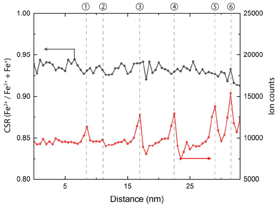
Figure S3: Charge-state ratio (CSR) analysis. CSR analysis of the superlattice system, using the Fe charge state (black line). The dashed lines indicate the position of the LuFe 2 O 4 layers, obtained by considering the ionic density profile (red line), which can detect very subtle changes to the electric field evaporation criteria. Importantly, the CSR analysis does not identify any substantial changes to the electric field strength, which rules out any major artefacts stemming from changes to the field evaporation criteria.
