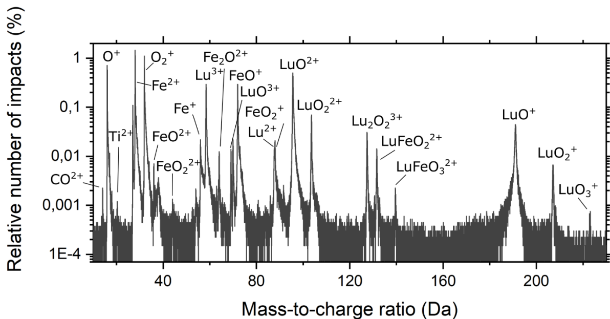
Figure S1: Mass spectrum of the (LuFeO_3)_9/(LuFe_2O_4)_1 superlattice. Figure shows the mass spectrum of the superlattice shown in Figure 1 in the main text. The spectrum is mainly coming from the thin film, but minor peaks from the substrate and capping layer are present, such as Ti^{2+} , which originates from the Ti protection layer. Species coming from the substrate are not labelled. In cases where peaks from the substrate and thin film overlap, the peak is assigned to the species belonging to the thin film. By integrating over the peaks, the average chemical composition from the thin film is found to be 53.74 \pm 0.04 at.% O, 23.78 \pm 0.05 at.% Lu and 22.56 \pm 0.05 at.% Fe.
