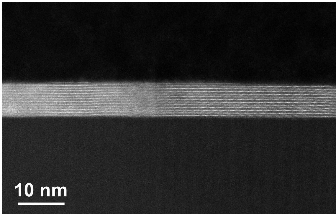
Figure S 3 - Low magnification cross-sectional HAADF-STEM of sample B showing an abrupt film-substrate interface.
