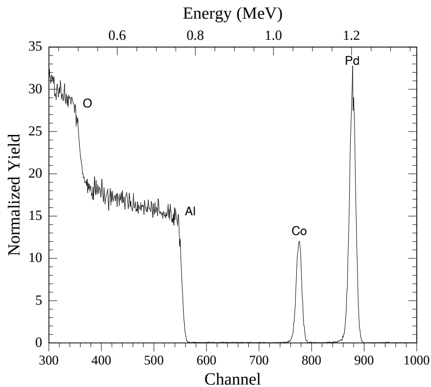
Figure S 5 - Rutherford backscattering spectrum (RBS) of sample B, an 8.0 nm thick PdCoO 2 film grown on (0001) sapphire. The Pd:Co ratio was found to be 1:1.05 indicating that the film is stoichiometric within the resolution of RBS.
