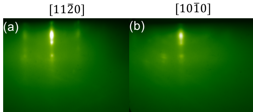
Figure S 4 - RHEED patterns of semi-crystalline films resulting from Pd-rich deposition condition. (a) and (b) are patterns taken along the two in-plane high symmetry directions indicated.
