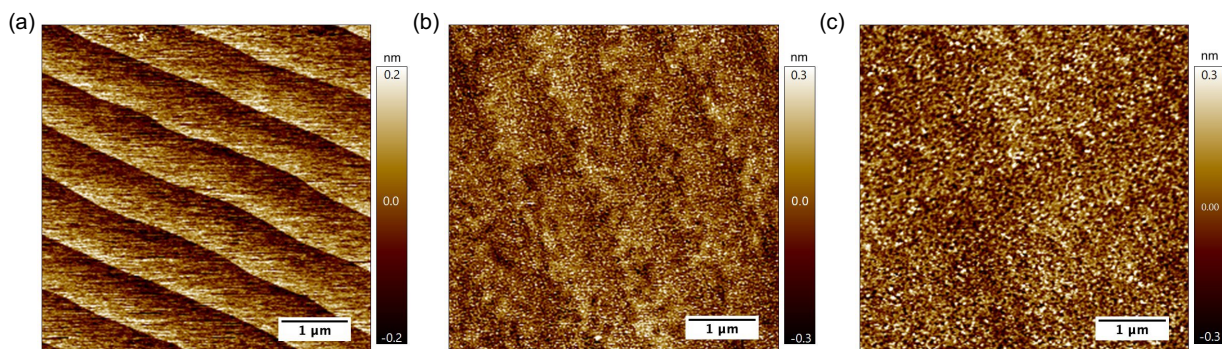
Figure S 1 – AFM images of (a) a bare (annealed) c -plane sapphire showing the step-and-terrace morphology with rms roughness of \sim 0.08 nm and (b) a similar c -plane sapphire substrate upon which Co-Pd-Co monolayers have been deposited. The \sim 0.6 nm thick PdCoO 2 film has completely coalesced while the substrate morphology underneath is still visible. The rms roughness is \sim 0.12 nm. (c) At end of the growth of an 8.0 nm thick PdCoO 2 film (sample B). The rms roughness is \sim 0.13 nm.
