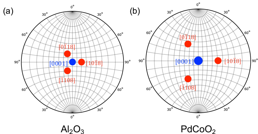
Figure S 2 - Stereographic projection of the 01•8 peak of single crystals of c -axis oriented (a) \text{Al}_2\text{O}_3 and (b) \text{PdCoO}_2 . In both cases three equivalent poles are present, i.e., three peaks are expected in the \phi scan for an untwinned single crystal of either of these materials.
