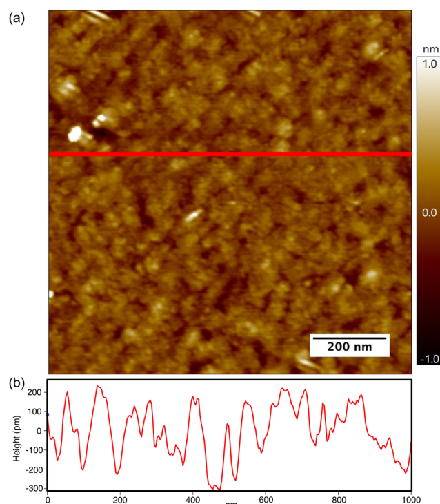
FIG. 2. AFM image of (a) sample B, an 8.0 nm thick PdCoO 2 film with a smooth surface morphology and a rms roughness of \sim 0.13 nm. (b) The height along a line profile corresponding to the red line drawn in (a).
