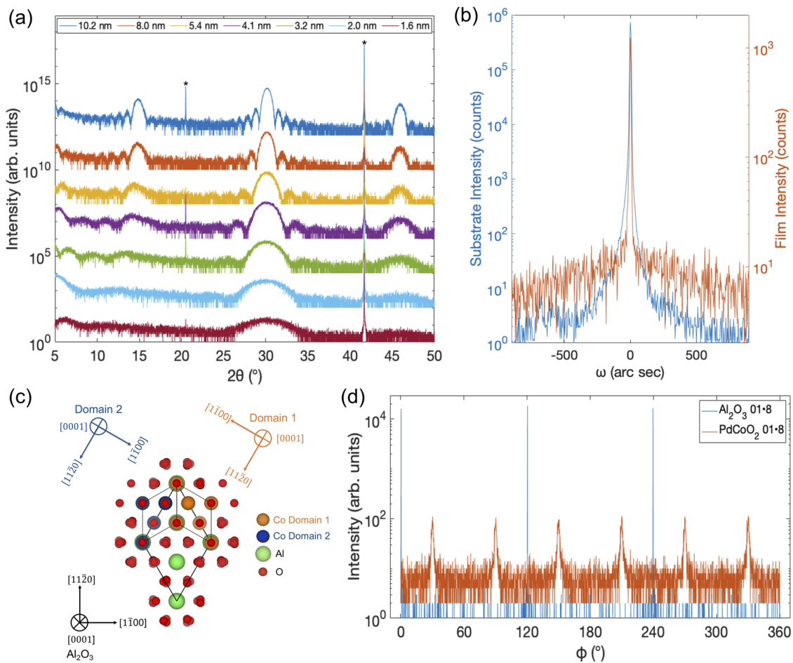
FIG. 3. X-ray diffraction (a) \theta - 2\theta scans of samples A-G showing only 000 \ell reflections of \text{PdCoO}_2 and Laue oscillations indicating an abrupt and smooth film-substrate interface. Asterisks (*) denote substrate reflections. The scans are vertically offset from each other for clarity. (b) Overlaid rocking curves in \omega of the 0006 film and substrate reflections of sample B; the comparable widths (9 arc sec for both the substrate and film) indicate low out-of-plane mosaicity. (c) In-plane epitaxial relationship between (0001) \text{PdCoO}_2 and (0001) \text{Al}_2\text{O}_3 showing the two \text{PdCoO}_2 domains with equivalent lattice mismatch with respect to \text{Al}_2\text{O}_3 and (d) off-axis \phi scan of 01·8 reflections of \text{PdCoO}_2 and \text{Al}_2\text{O}_3 of sample A showing three poles for the substrate, but six poles for the film due to 180^\circ in-plane rotation twinning.
