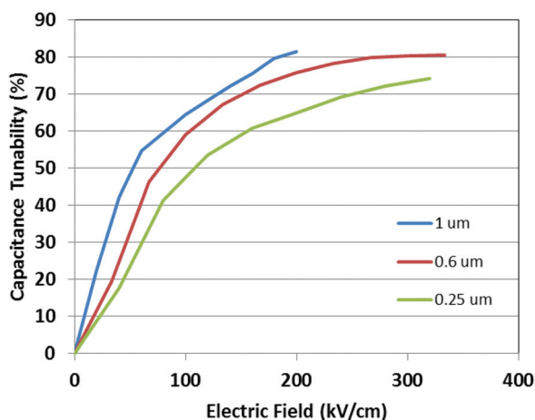
FIG. 34. Thickness dependence of capacitance tunability vs. electric-field for 5\text{ }\mu\text{m} \times 5\text{ }\mu\text{m} size varactor. Reproduced by permission from Subramanyam et al. , Integr. Ferroelectr. 112 , 53 (2009). Copyright 2009 by Taylor & Francis.
