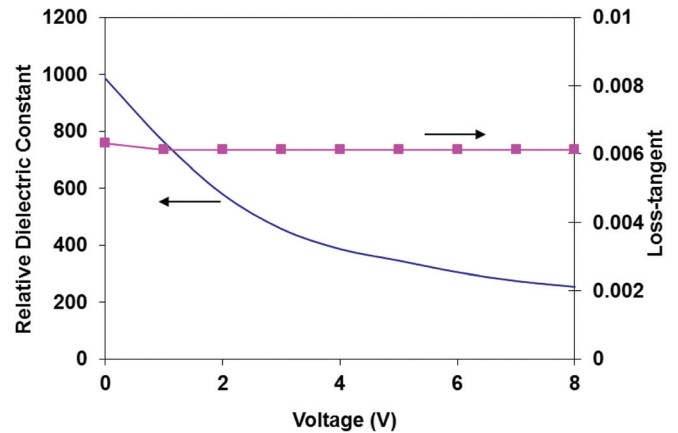
FIG. 2. The dielectric properties of the 0.25\ \mu\text{m} thick BST thin film on a 4 in. R-cut sapphire substrate. The dielectric properties were obtained by matching measured scattering parameters of a varactor device to an electrical model over a wide frequency range. The dielectric loss-tangent shown is calculated at 10 GHz. Reproduced by permission from Subramanyam et al. , IEEE Trans. Ultrason. Ferroelectr. Freq. Control 57 , 1692 (2010). Copyright 2010 by IEEE.
