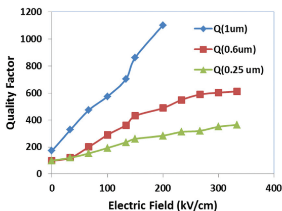
FIG. 35. Quality factor vs. electric field for 5 \times 5\text{ }\mu\text{m}^2 varactors fabricated using 3 different thicknesses of BST layers. The Q was computed at 1 GHz. Reproduced by permission from Subramanyam et al. , Integr. Ferroelectr. 112 , 53 (2009). Copyright 2009 by Taylor & Francis.
