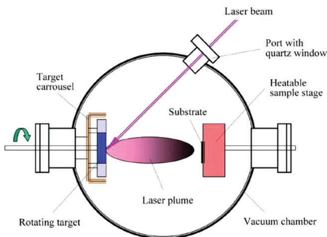
FIG. 6. Schematic diagram of a typical PLD system (Reprinted from source: http://www.andor.com/Portals/0/Pulsed%20Laser%20Deposition.jpg ).
