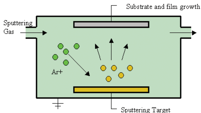
FIG. 7. Schematic diagram of a typical sputtering system. Diagram depicts a "sputter-up" configuration.
