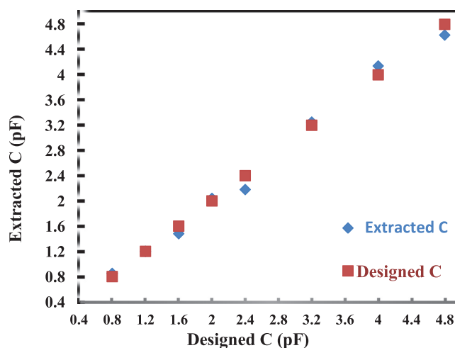
FIG. 42. Comparison of the extracted device capacitance at 0-V to the design capacitance on low-resistivity CMOS Si. The extracted capacitance is obtained by matching the S-parameters of the measured devices to the S-parameters of the device equivalent circuit model.
