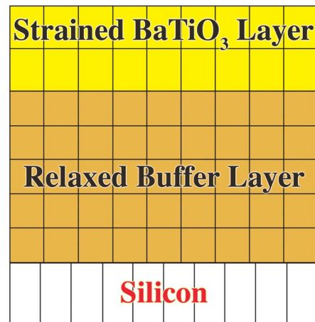
FIG. 2. (Color online) A schematic of the structure used for the growth of epitaxial c -axis BaTiO 3 on Si (001). The structure involves the presence of a completely relaxed buffer layer between the silicon and the ferroelectric BaTiO 3 . The thickness of the epitaxial BaTiO 3 should be below its critical thickness.
